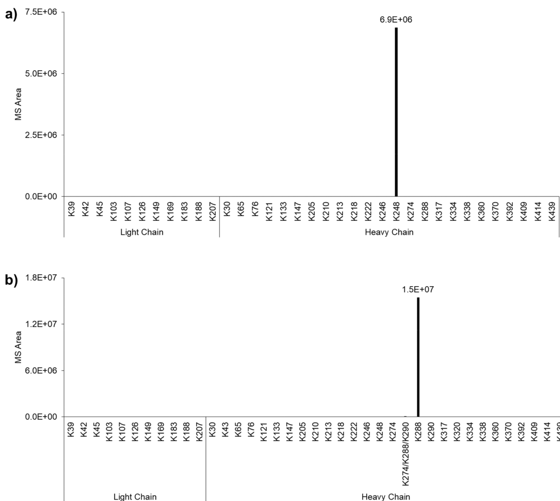
Figure 2. Summary of lysine residue search by BioPharma Finder: (a) analysis of trastuzumab-Lys248-thiol (4a); (b) analysis of trastuzumab-Lys288-thiol (4b). Each result shows the high specificity of the AJICAP reaction.
